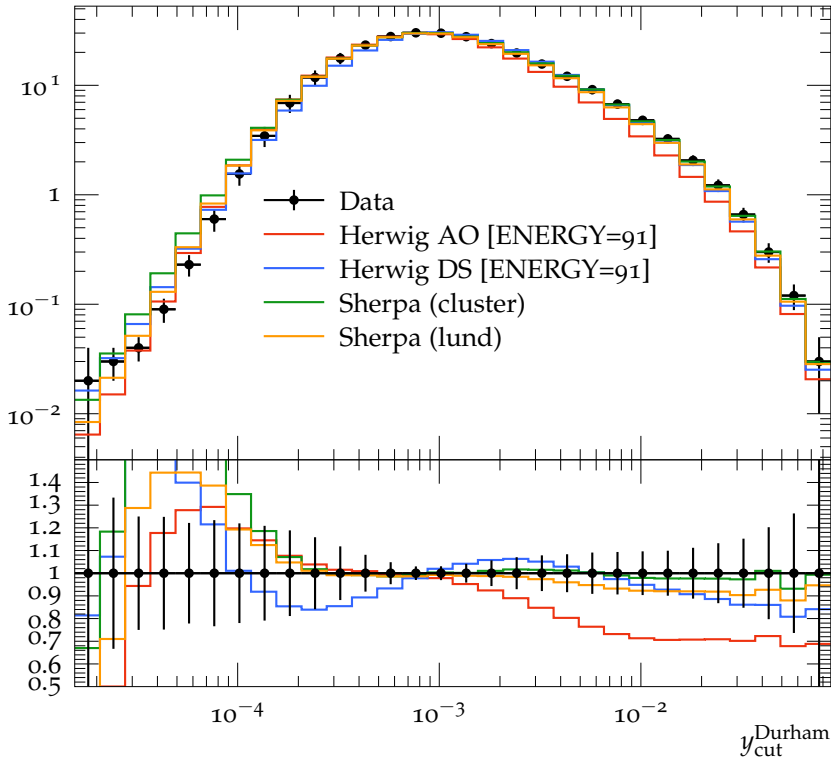
Integrated 4-jet rate with Durham algorithm (91.2 GeV)
