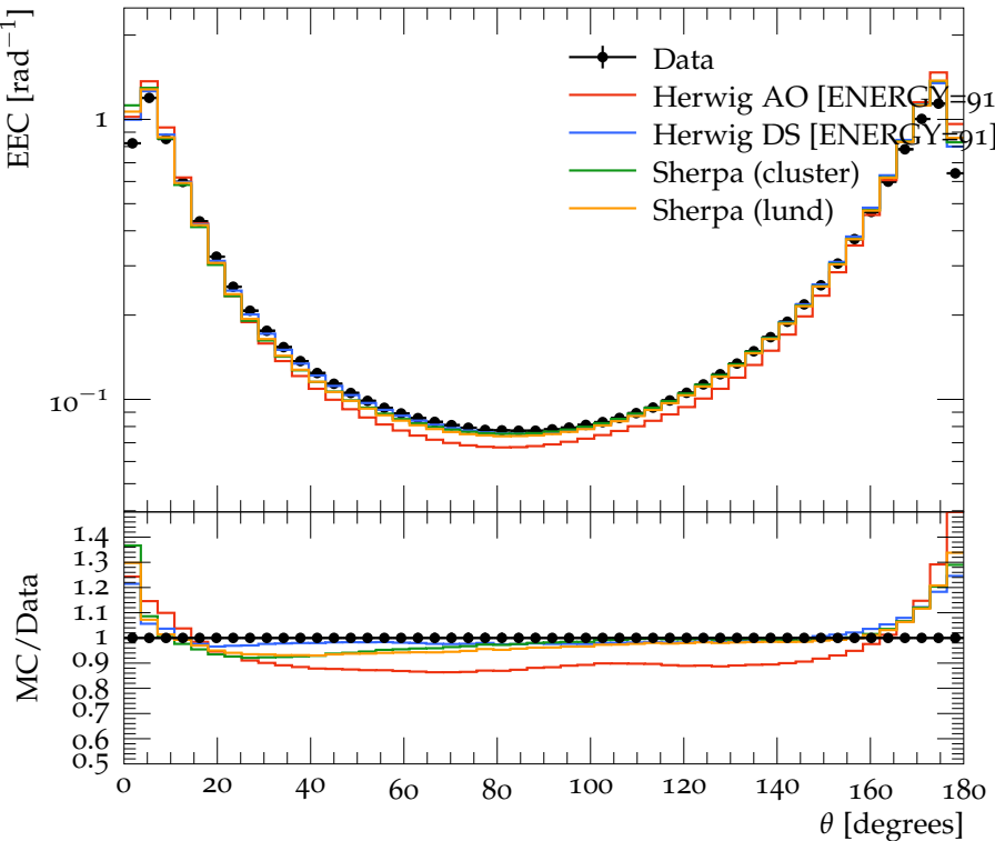
EEC for all \cos \theta_T
