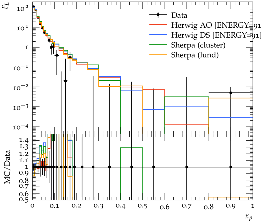
Longitudinal charged particle fragmentation function (uds)
