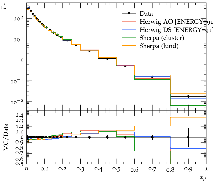
Transverse charged particle fragmentation function
