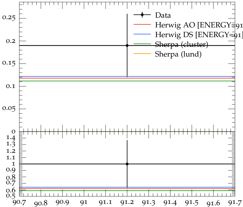
Mean K_2^*(1430)^0 multiplicity
