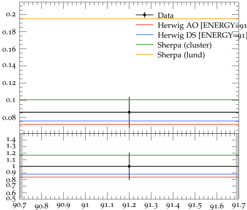
Mean \phi multiplicity
