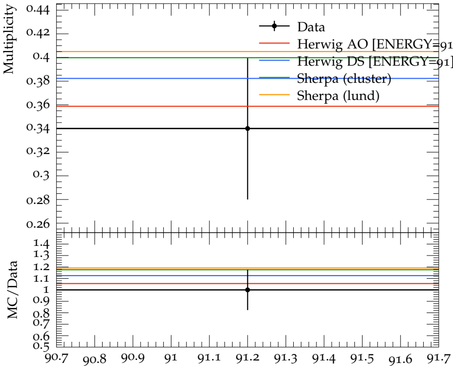
Mean B^+ / B^- / B^0 multiplicity
