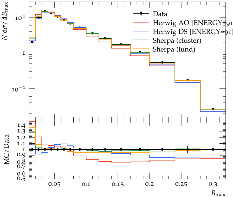
Wide hemisphere broadening, B_{\max}
