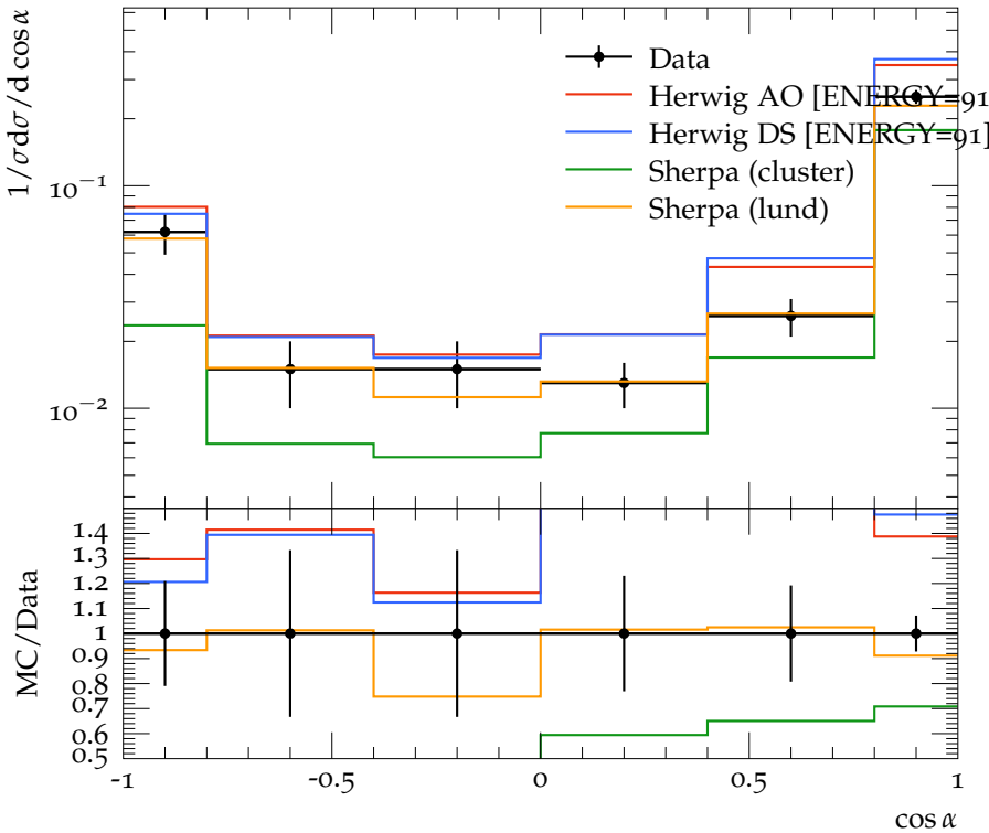
Cosine of the angle between \Lambda^0 and \bar{\Lambda}^0
