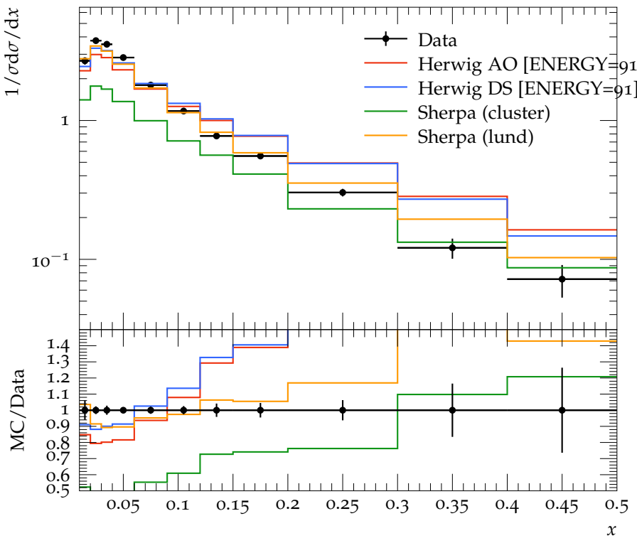
\Lambda^0, \bar{\Lambda}^0 scaled momentum spectrum
