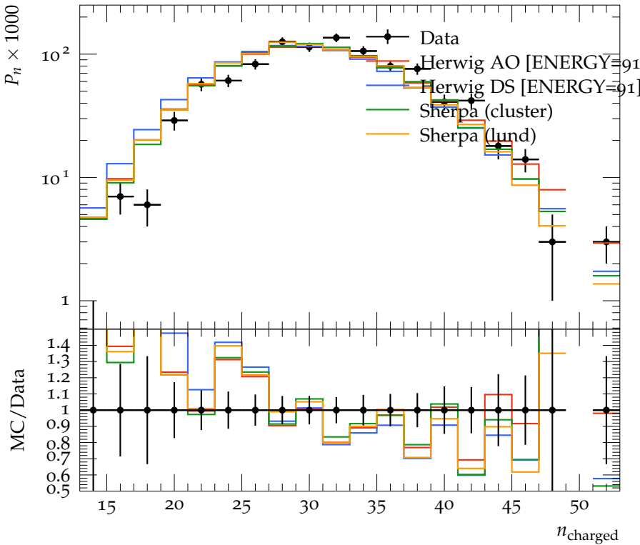
Charged particle multiplicity, 4-jets, y_{\text{cut}} = 0.04
