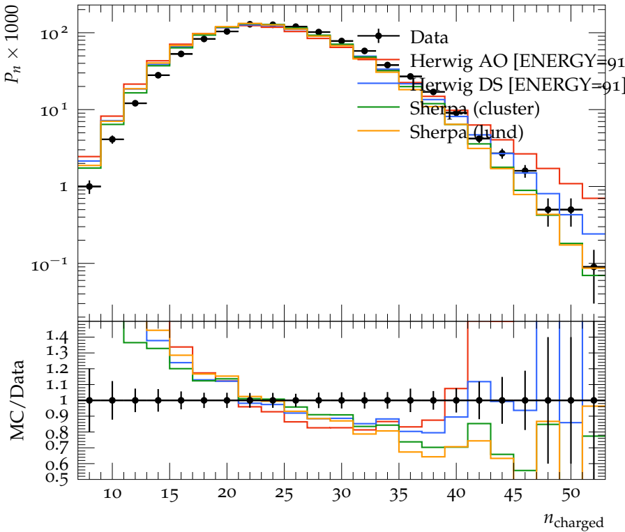
Charged particle multiplicity, 3-jets, y_{\text{cut}} = 0.04
