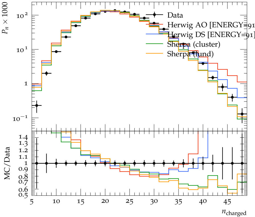
Charged particle multiplicity, 3-jets, y_{\text{cut}} = 0.02
