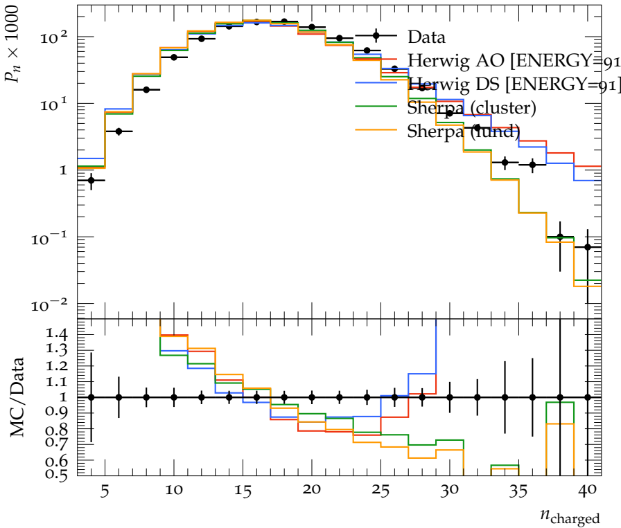
Charged particle multiplicity, 2-jets, y_{\text{cut}} = 0.01
