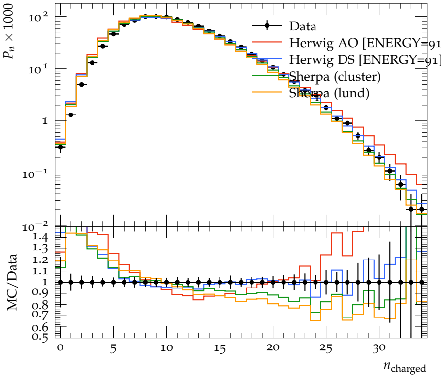
Charged Particle Multiplicity, single hemisphere, |y| < 5.0
