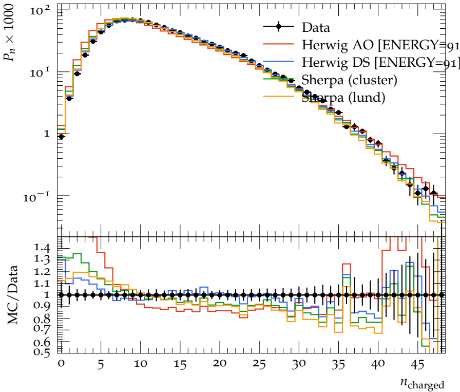
Charged Particle Multiplicity, both hemispheres, |y| < 2.0
