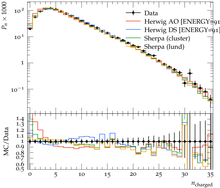
Charged Particle Multiplicity, both hemispheres, |y| < 1.0
