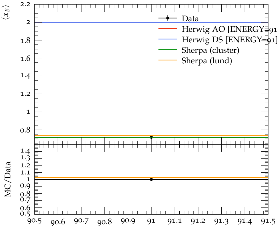
Mean of b quark fragmentation function f(x_B^{\text{weak}})
