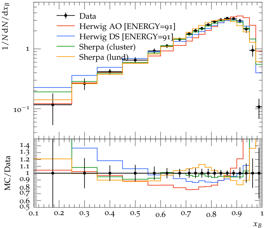
b quark fragmentation function f(x_B^{\text{lead}})
