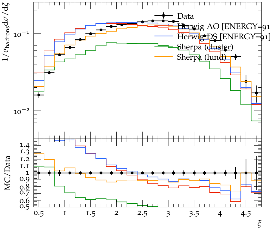
Log Scaled momentum fraction for \Lambda^0 (all events)
