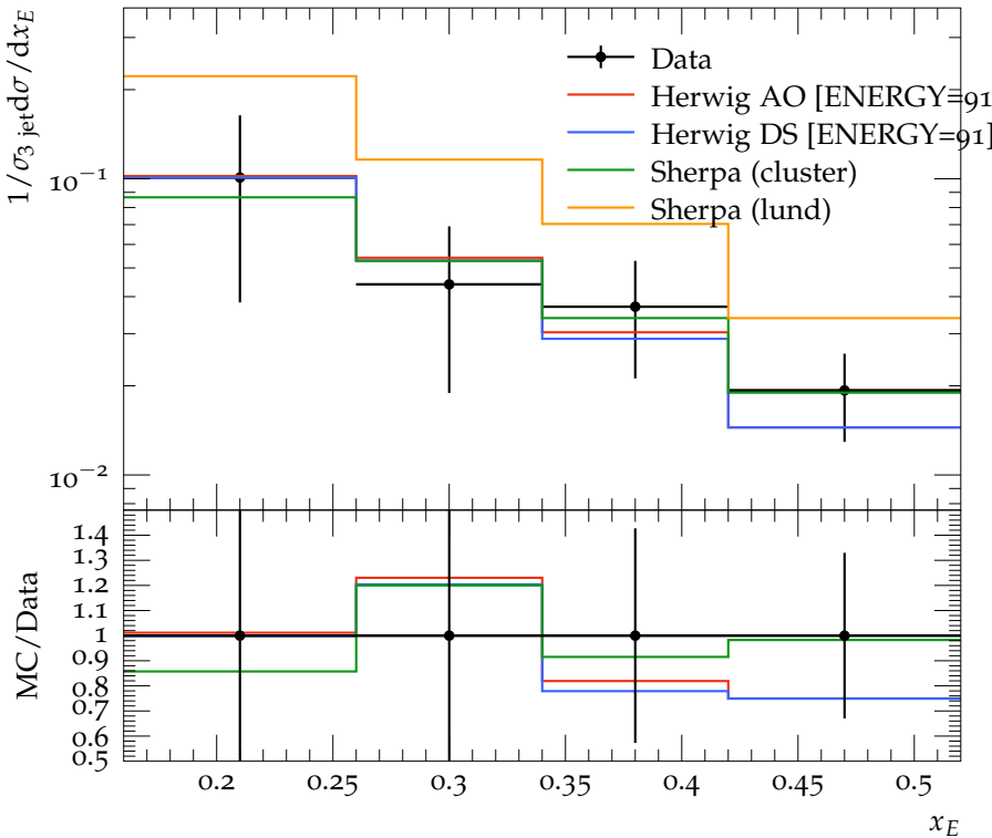
Scaled energy fraction for \eta' in 1st jet (3-jet events)
