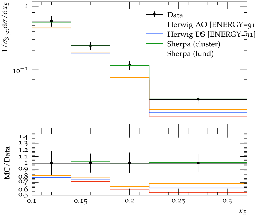
Scaled energy fraction for \eta in 3rd jet (3-jet events)
