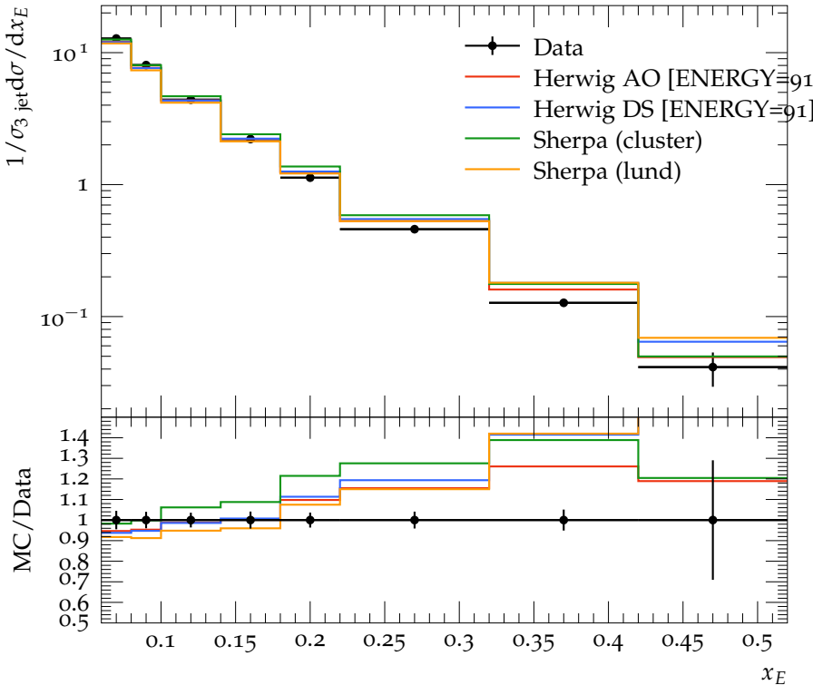
Scaled energy fraction for \pi^0 in 2nd jet (3-jet events)
