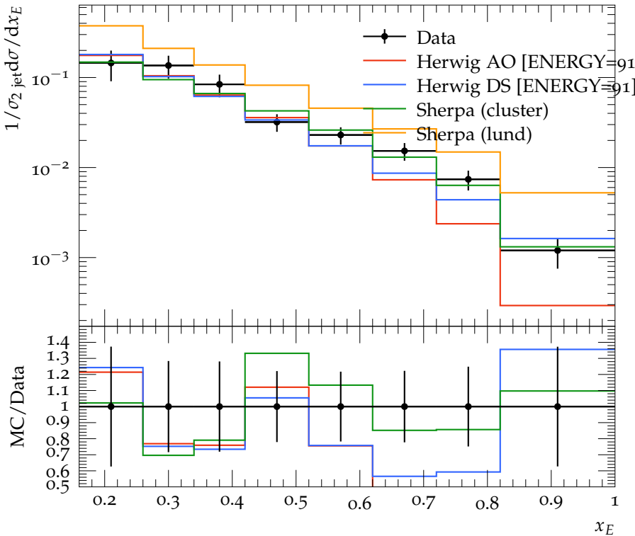
Scaled energy fraction for \eta' (2-jet events)
