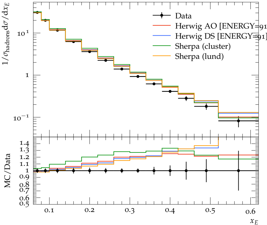
Scaled energy fraction for \pi^0 (all events)
