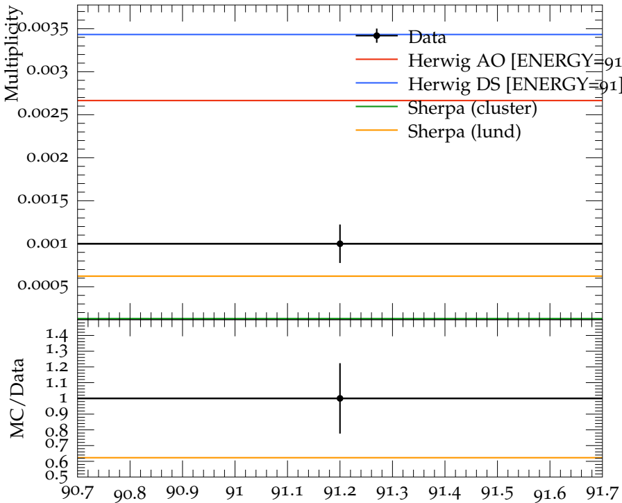
Mean \Omega^\mp multiplicity
