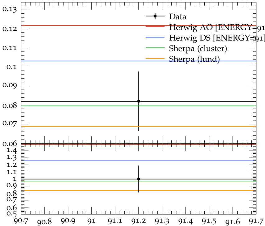
Mean \Sigma multiplicity
