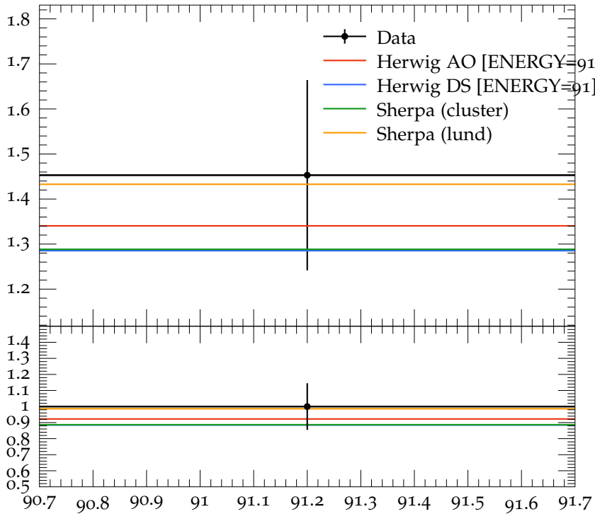
Mean \rho^0 multiplicity
