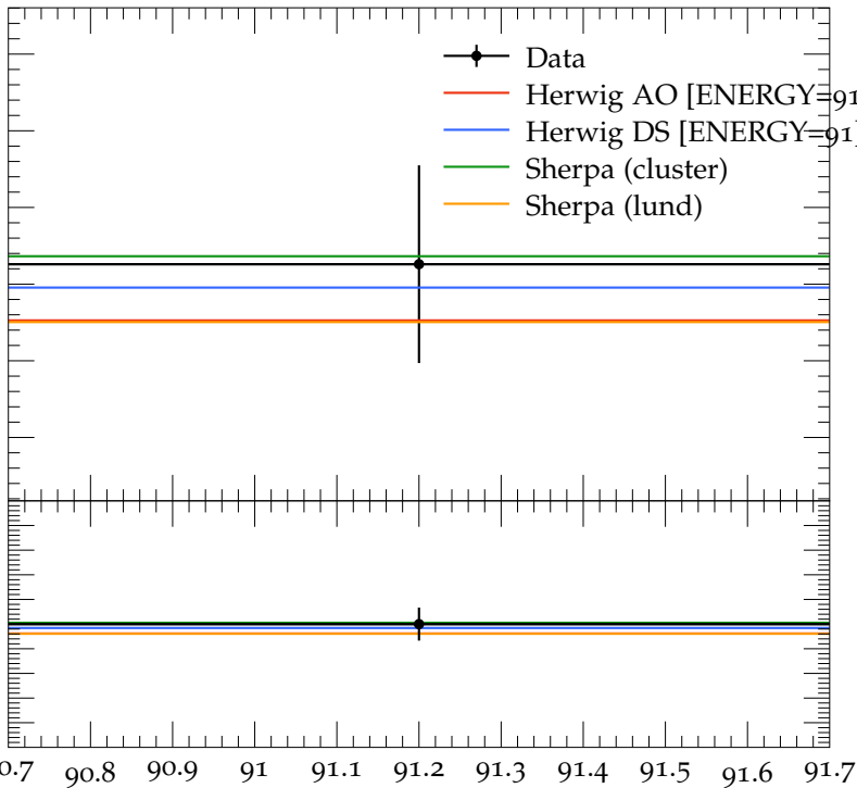
Mean \pi^0 multiplicity
