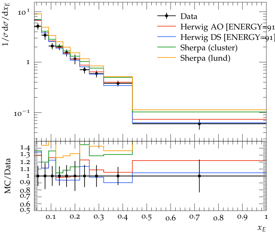
K^{*\pm}(892) spectrum
