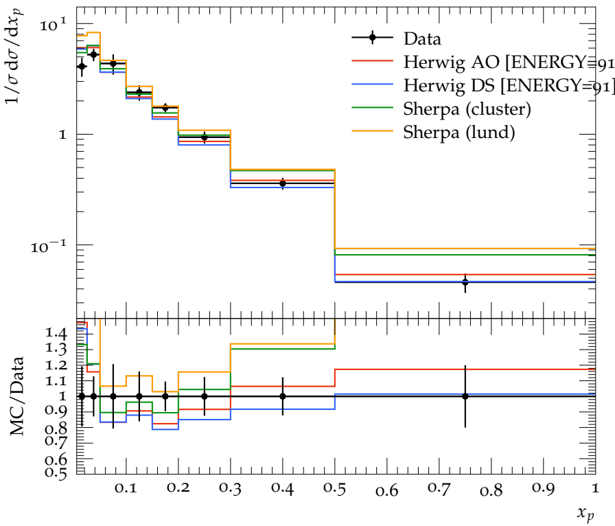
K^{*0}(892) spectrum
