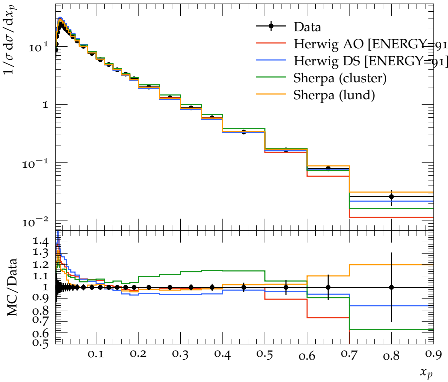
K^0 spectrum
