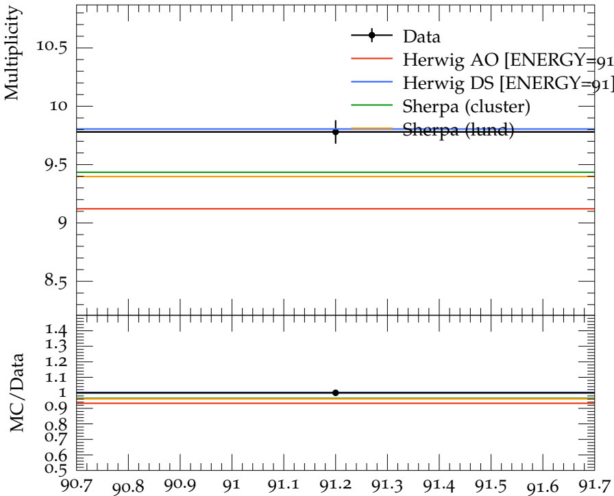
Mean charged multiplicity for rapidity |Y| < 1.5
