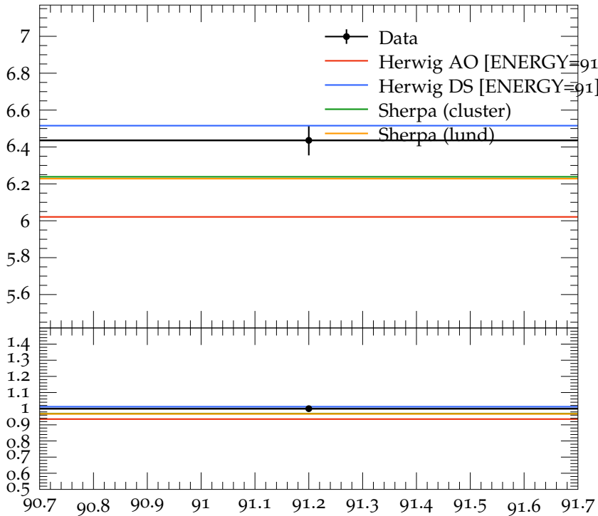
Mean charged multiplicity for rapidity |Y| < 1.0
