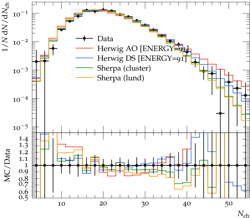
Charged multiplicity distribution
