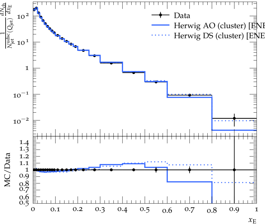
udsc hemisphere jet fragmentation, at 91.2 GeV
