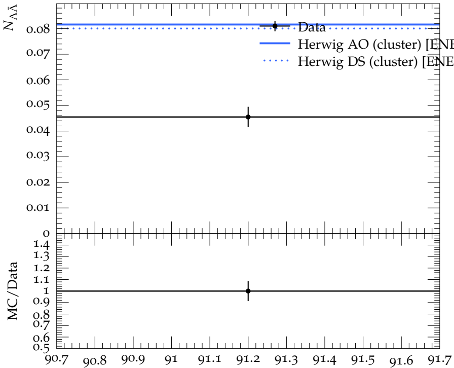
\Lambda\bar{\Lambda} correlated pair multiplicity (2 jet events)
