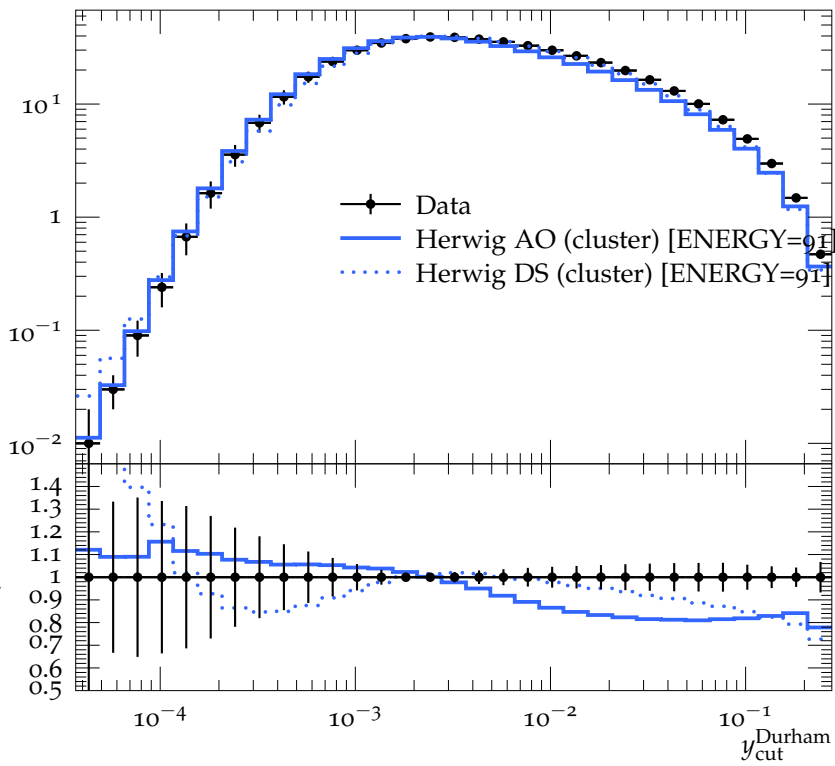
Integrated 3-jet rate with Durham algorithm (91.2 GeV)
