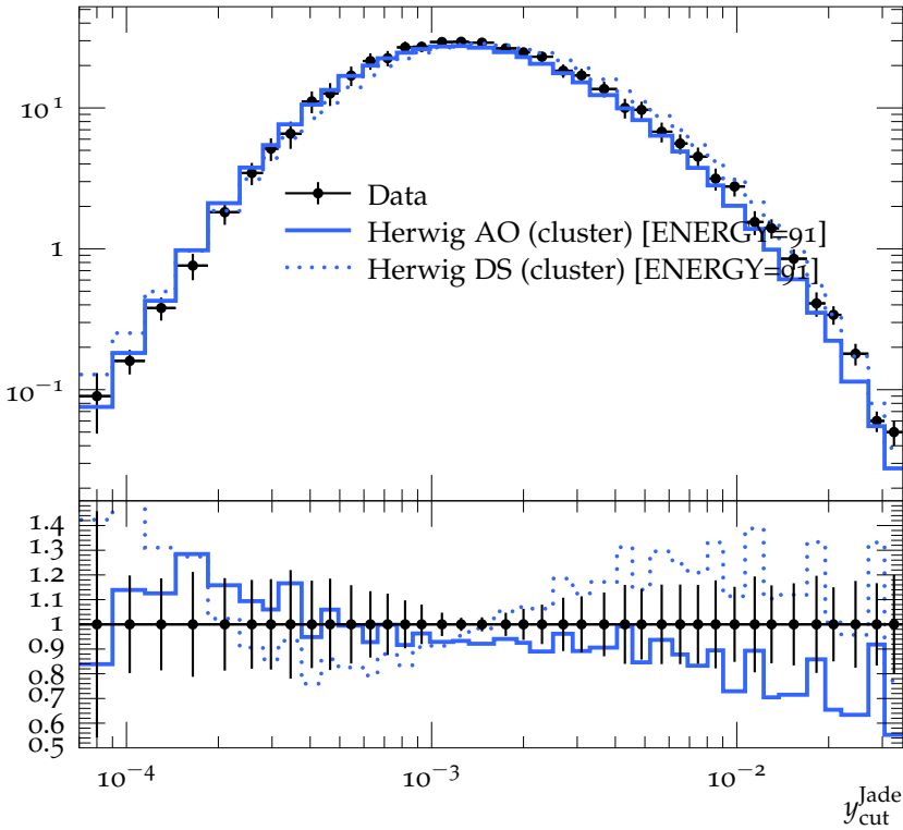
Integrated 5-jet rate with Jade algorithm (91.2 GeV)
