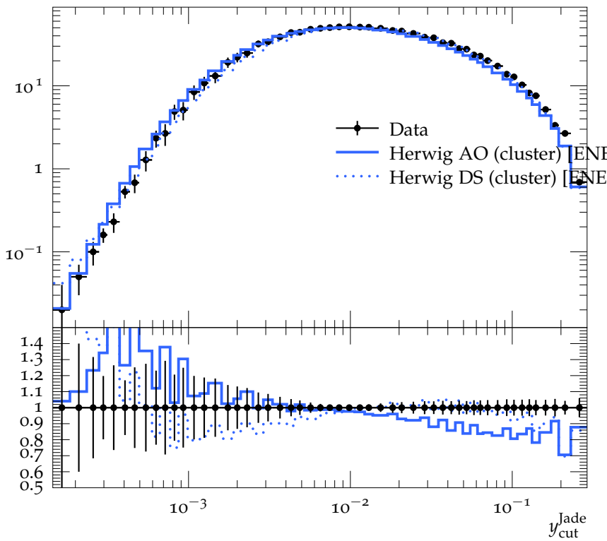
Integrated 3-jet rate with Jade algorithm (91.2 GeV)
