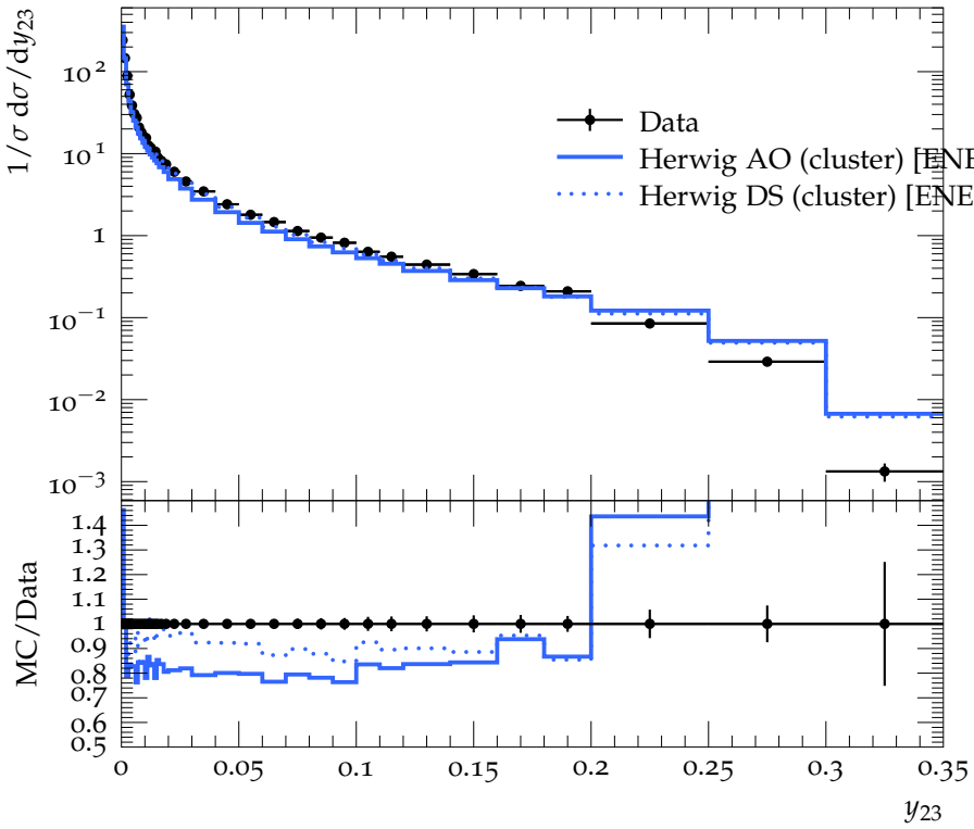
Differential 2-jet rate(Cambridge)
