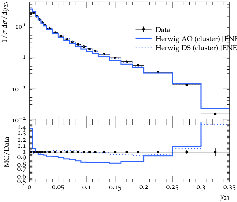
Differential 2-jet rate(JADE)
