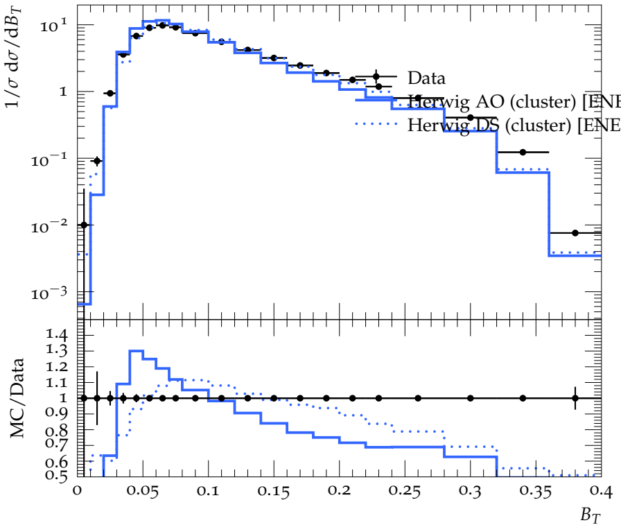
Total jet broadening
