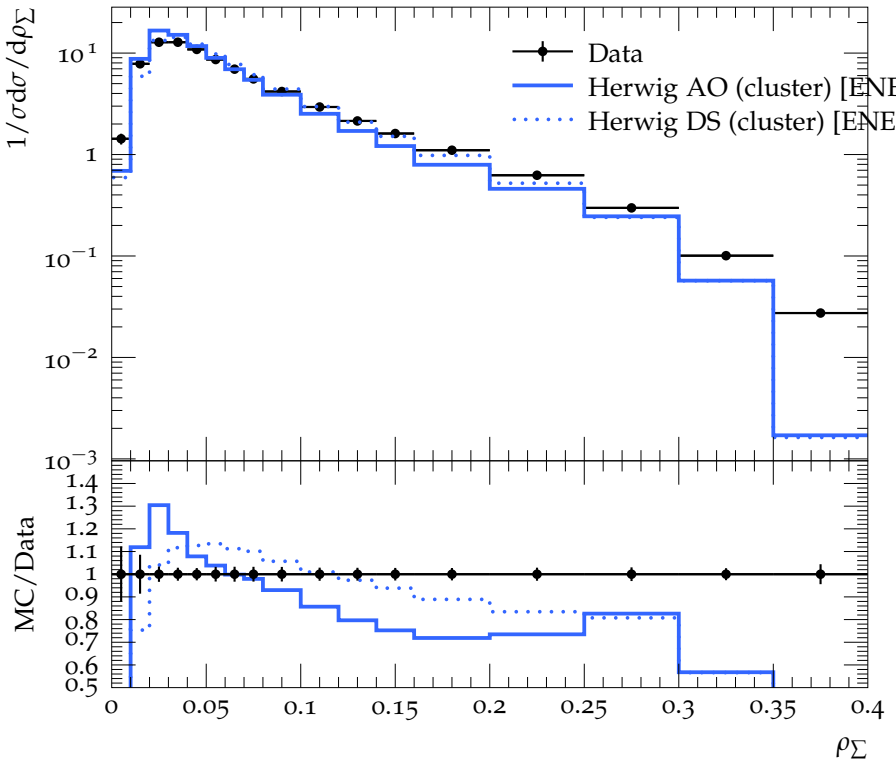
Sum of Jet Masses
