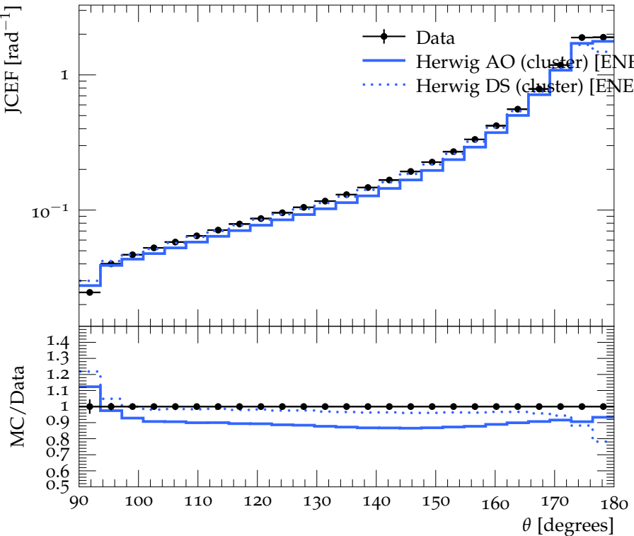
Jet Cone Energy Fraction for all \cos \theta_T
