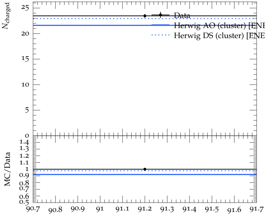
Charged Particle Multiplicity (bottom)
