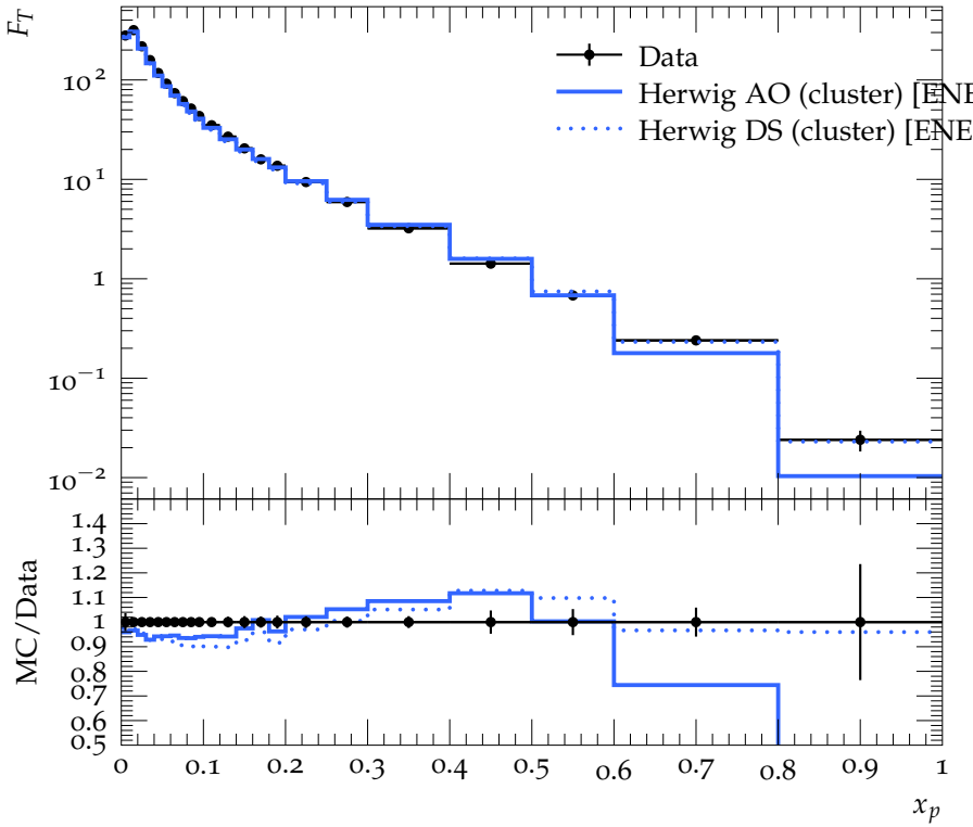
Transverse charged particle fragmentation function (uds)
