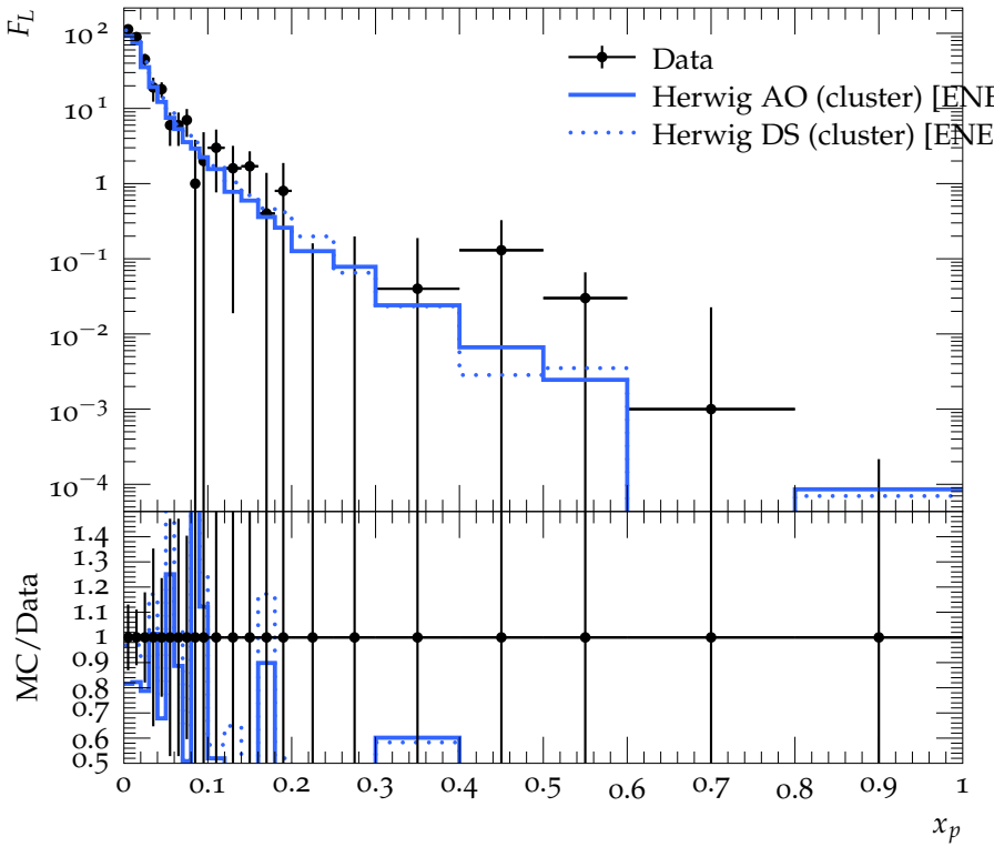
Longitudinal charged particle fragmentation function (bottom)
