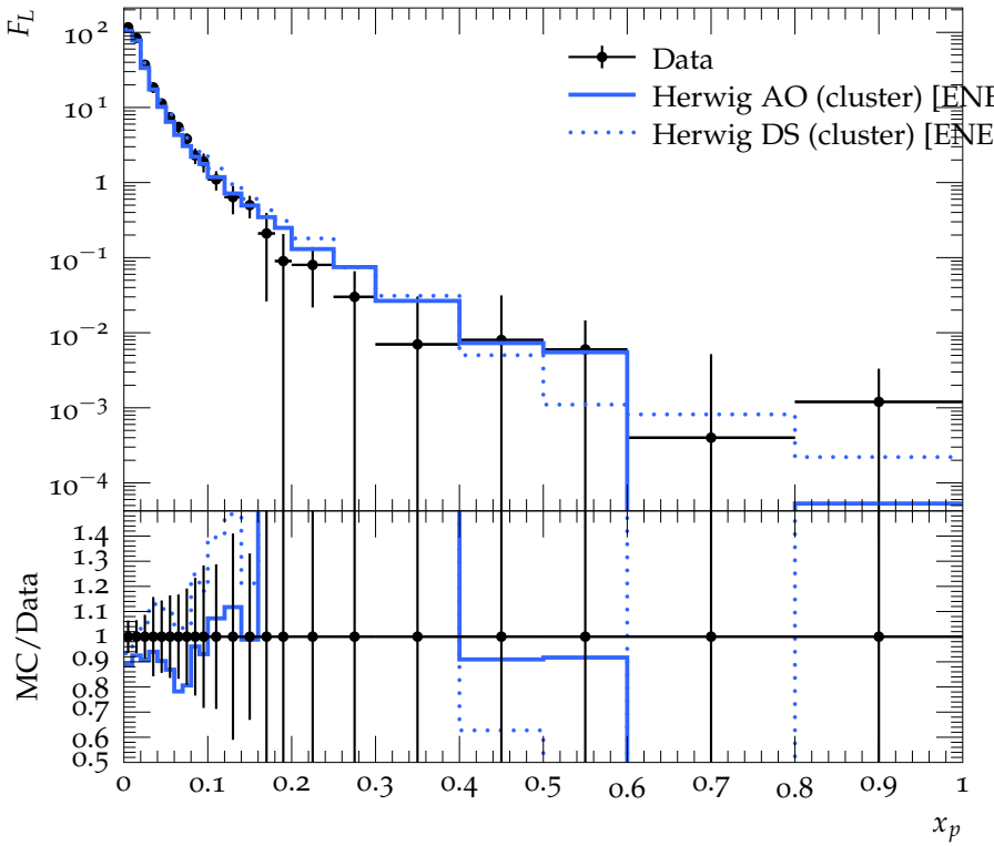
Longitudinal charged particle fragmentation function
