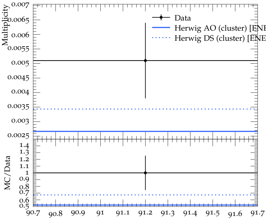
Mean \Omega^- multiplicity
